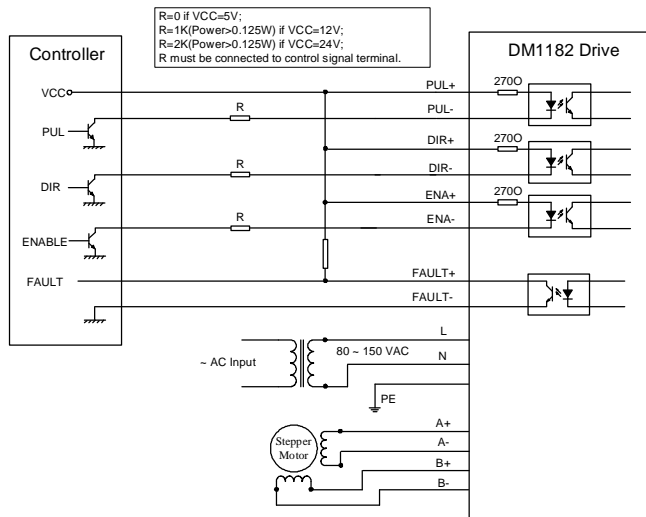
Figure 9: Typical connection
